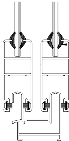
OUTER DETAIL
